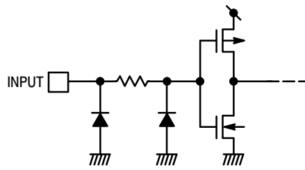
Figure 5. Input Equivalent Circuit
