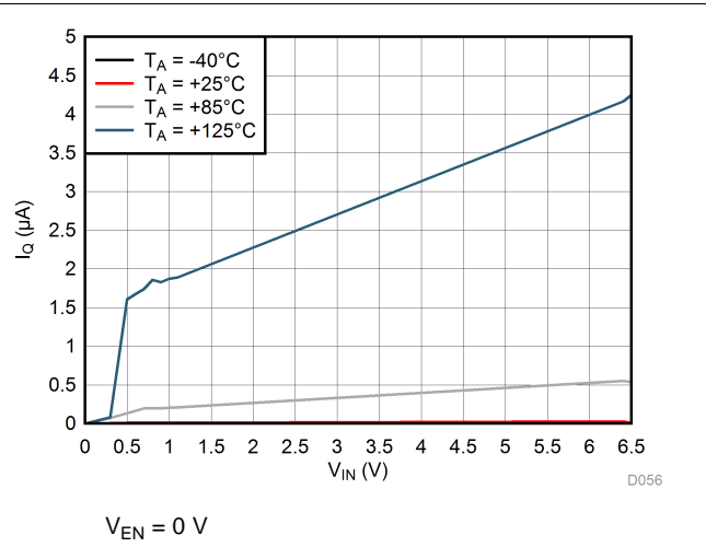
Figure 16. LP5912-3.3 I_{Q(SD)} vs V_{IN}
