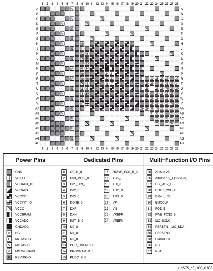
Figure 3-82: SFVB784 Package—XCKU3P and XCKU5P and SFRB784 Package—XQKU5P Configuration/Power Diagram
