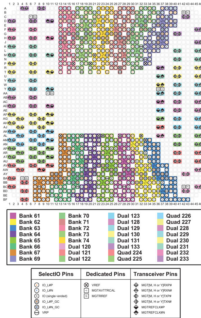
Figure 3-139: FIGD2104 Package—XCVU29P I/O Bank Diagram
