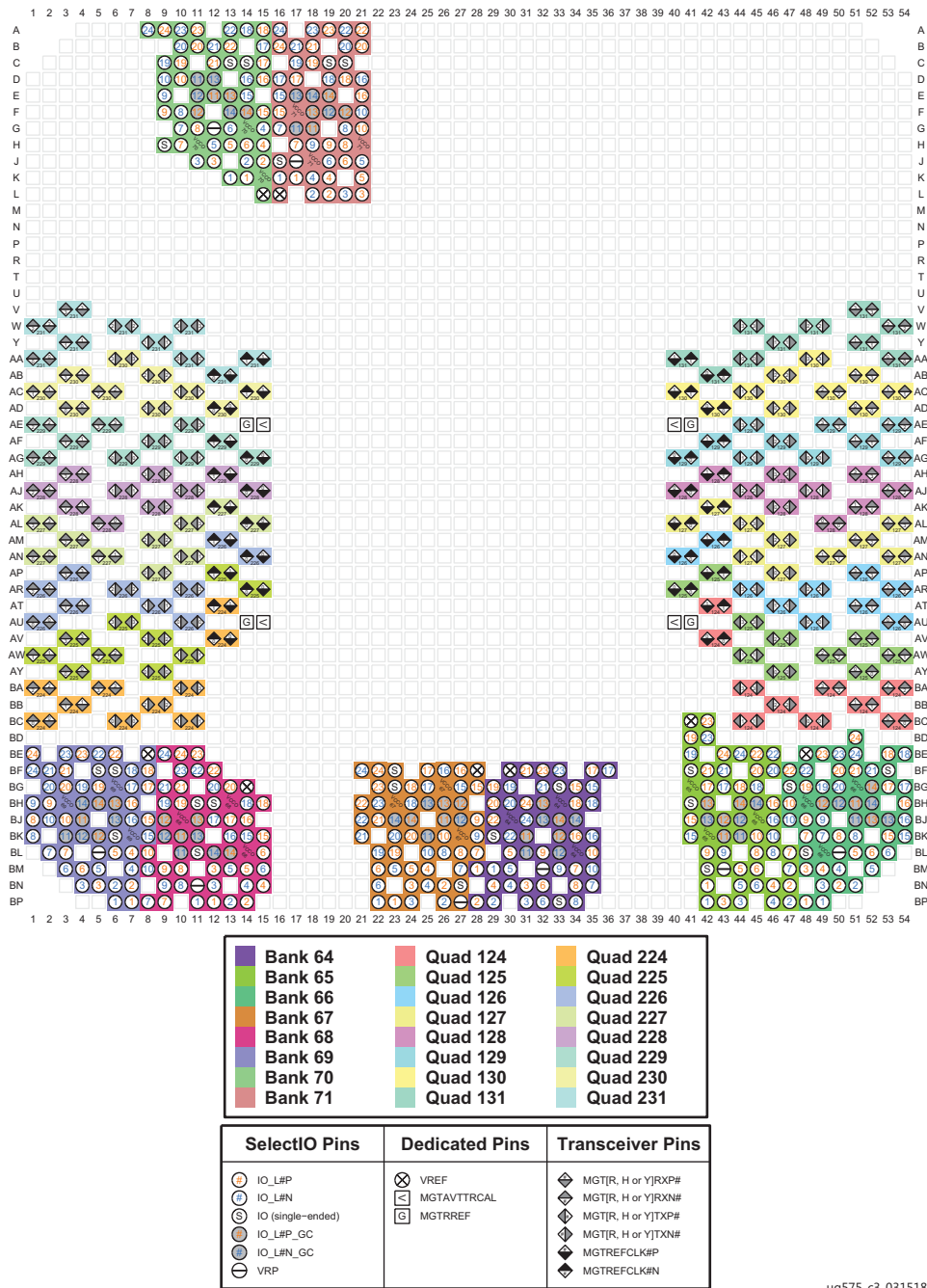
Figure 3-155: FSVH2892 Package—XCVU35P I/O Bank Diagram
