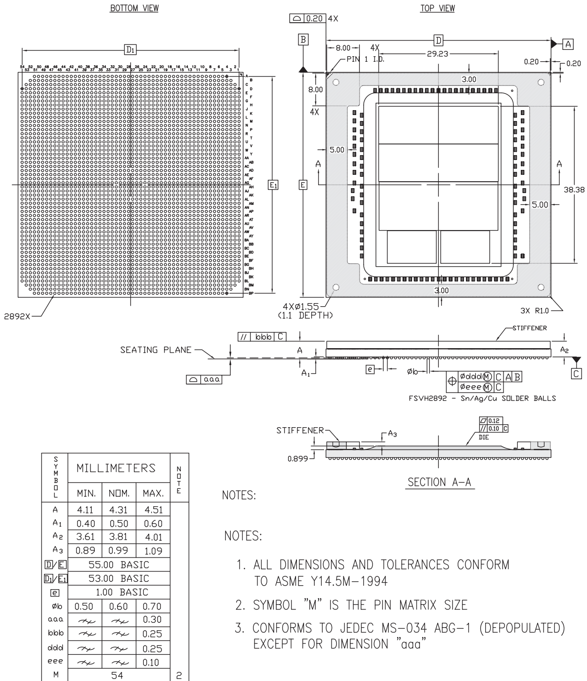
Figure 4-57: Package Dimensions for FSVH2892 (XCVU37P)
