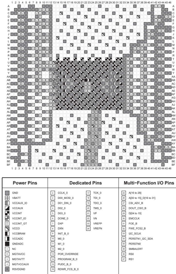
Figure 3-152: FSGA2577 Package—XCVU27P Configuration/Power Diagram
