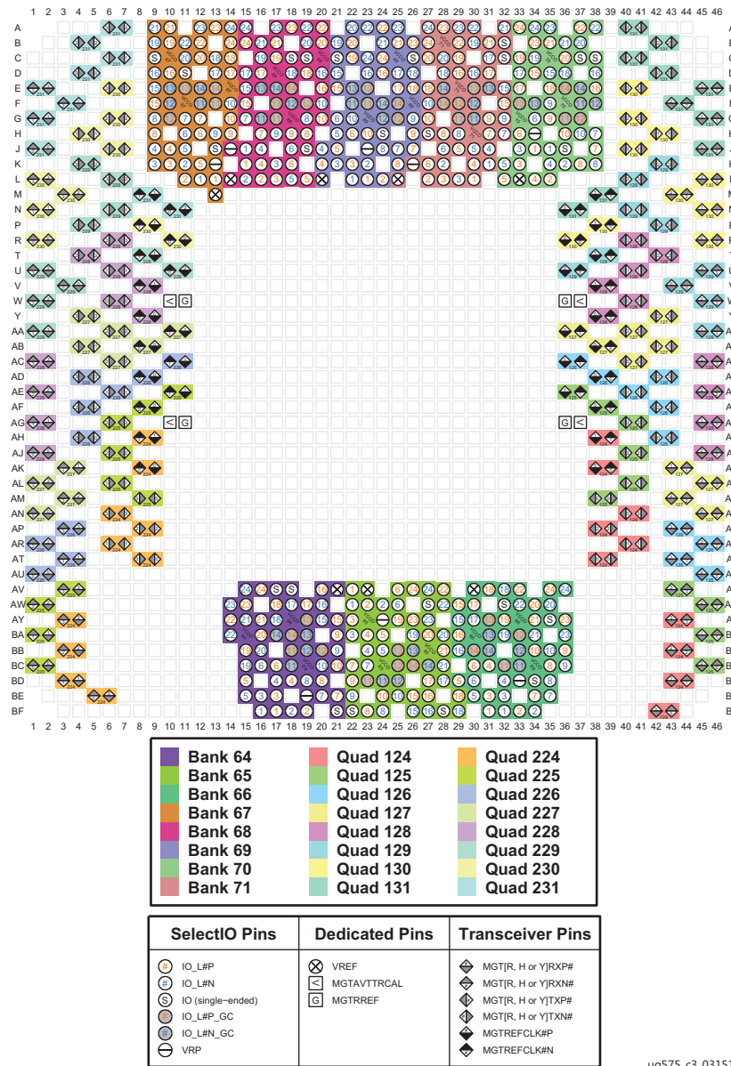
Figure 3-143: FSVH2104 Package—XCVU35P I/O Bank Diagram
