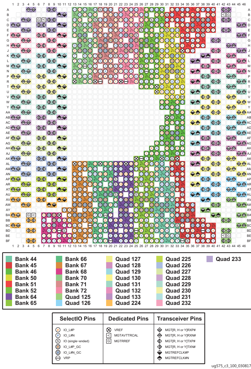
Figure 3-115: FLVB2104 Package—XCVU5P and XCVU7P and FLRB2104 Package—XQVU7P I/O Bank Diagram
