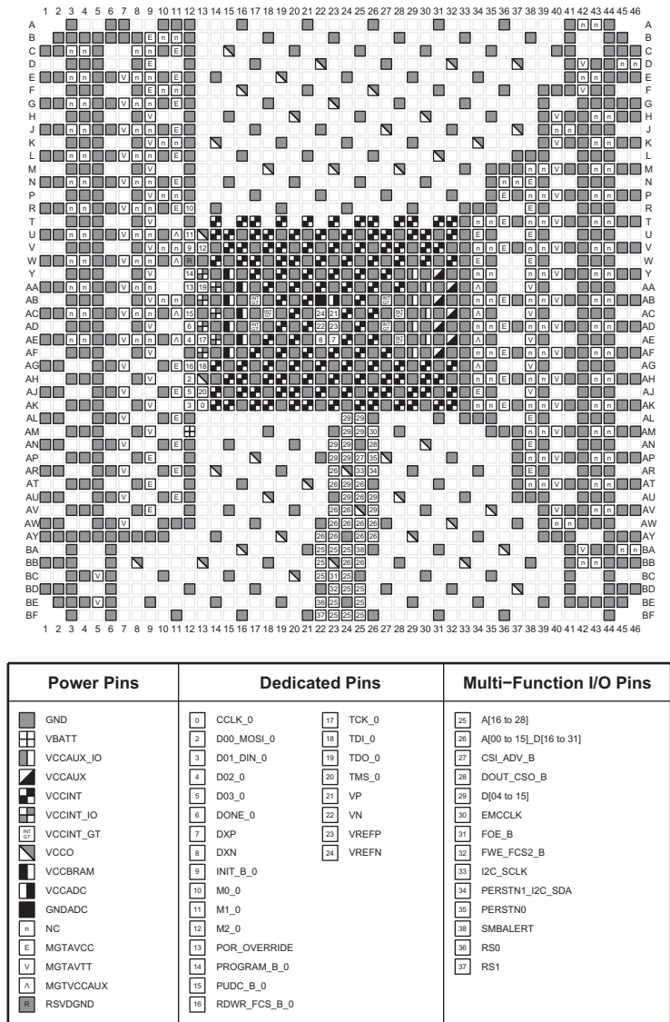
Figure 3-138: FIGD2104 Package—XC7VU27P Configuration/Power Diagram
