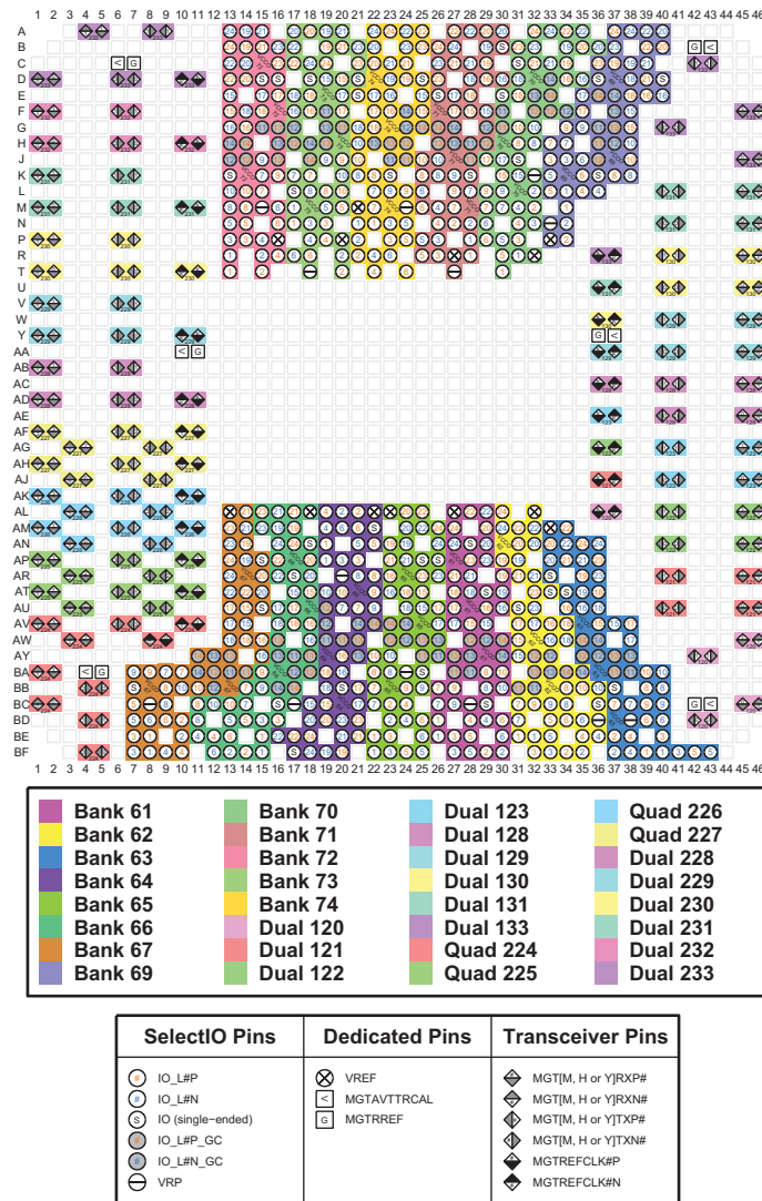
Figure 3-151: FSGA2577 Package—XCVU27P I/O Bank Diagram
