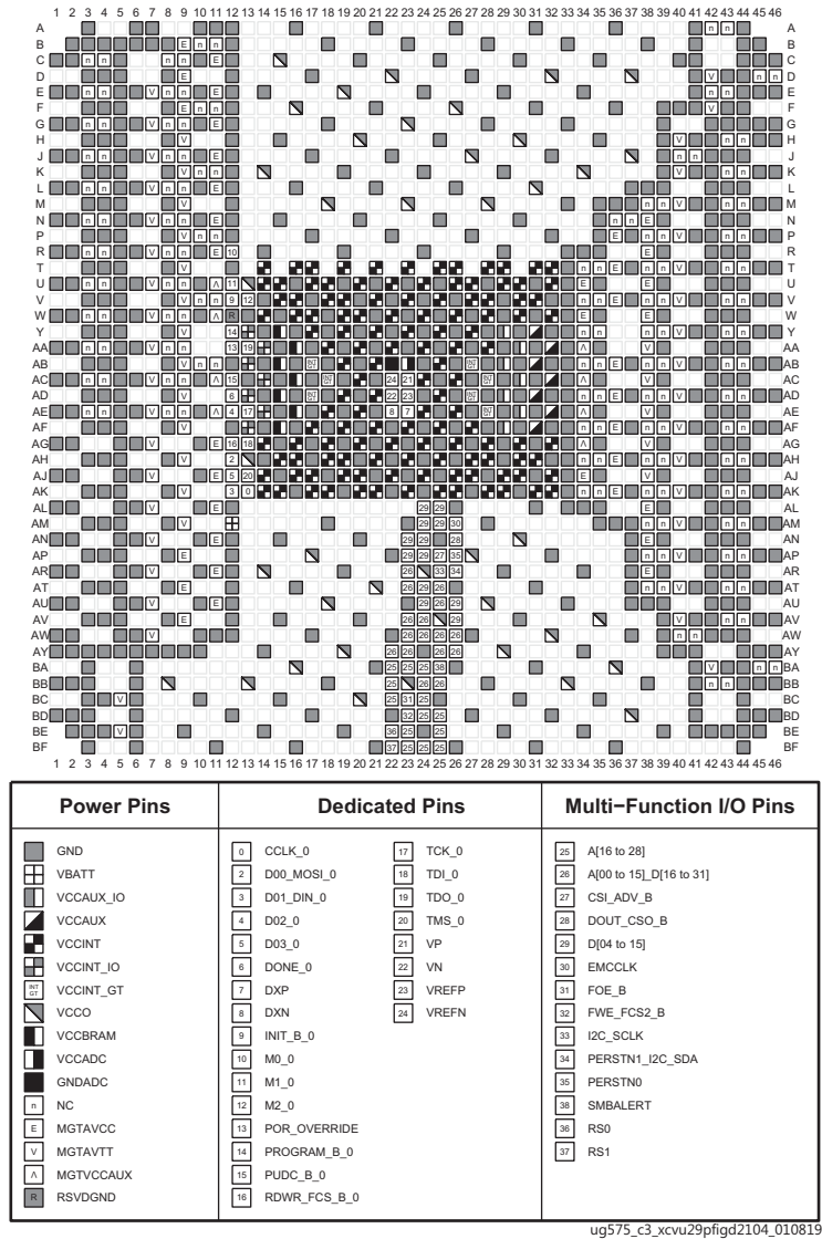
Figure 3-154: FSGA2577 Package—XCVU29P Configuration/Power Diagram
