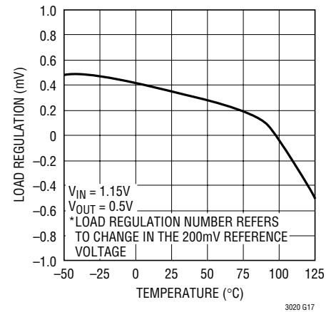
Load Regulation \Delta I_L = 1mA to 100mA
