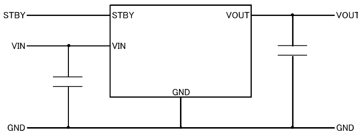
Figure 1. Application Circuit
