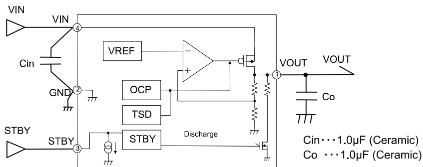
Figure 2. Block Diagrams
