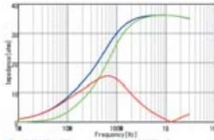
BLM18KG300TZ1/BLM18KG300TH1
