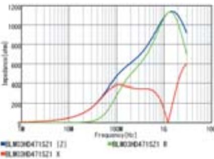
BLM03HD471SZ1
