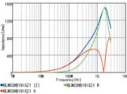
BLM03HB191SZ1
