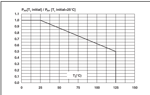
Figure 2. Relative variation of peak pulse power versus initial junction temperature (8/20 \mu s, typical values)
