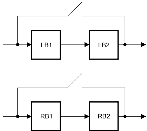
Figure 12. Structure of Digital Effects Processing for Independent Channel Processing
