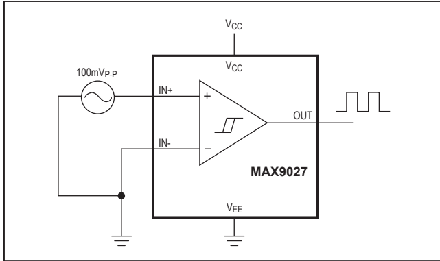
Figure 4. Zero-Crossing Detector
