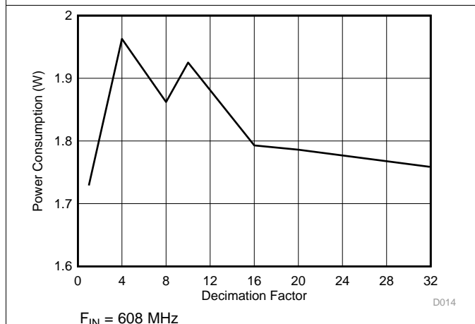
Figure 25. Power Consumption vs Decimation Setting
