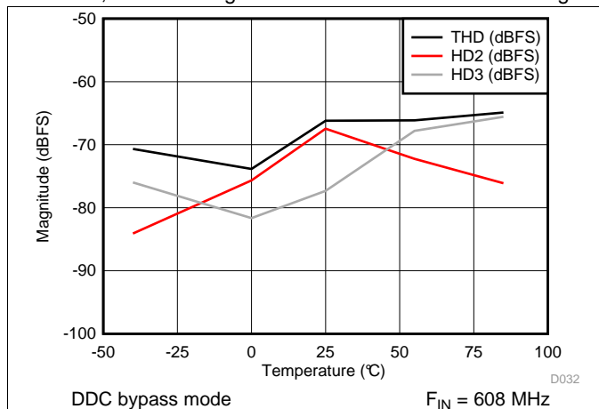
Figure 21. THD, H2, H3 vs Temperature - F_{IN} = 607.77\text{MHz}
