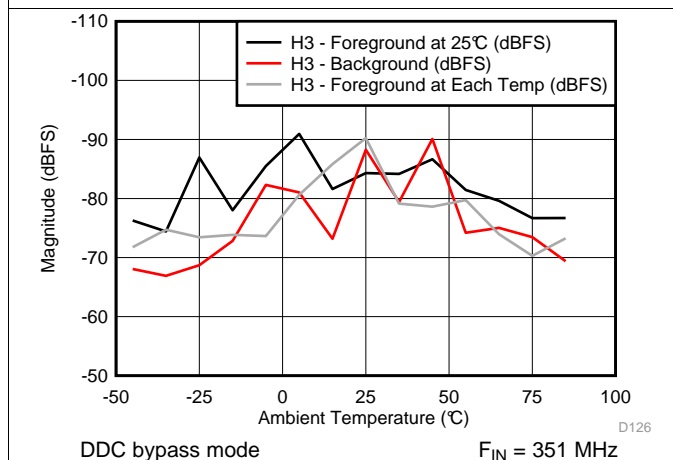
Figure 23. H3 vs Temperature and Calibration Mode
